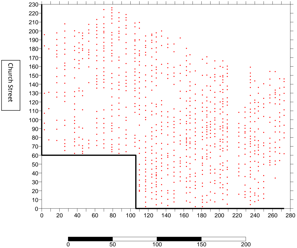
Ground Penetrating Radar Results Eastmanville Cemetery Polkton Township, Michigan
